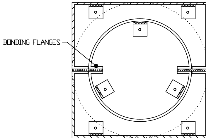
BASE ATTACHMENT DETAIL
