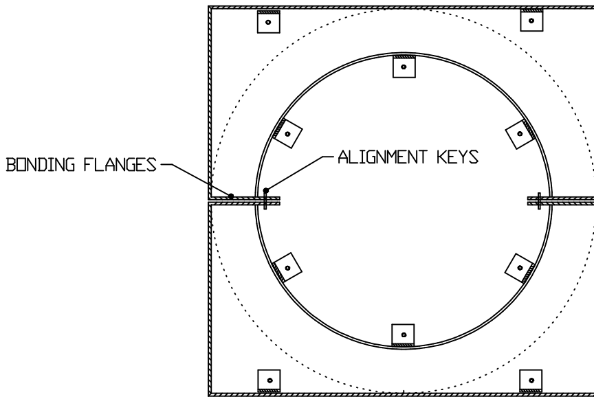
BASE ATTACHMENT DETAILS
