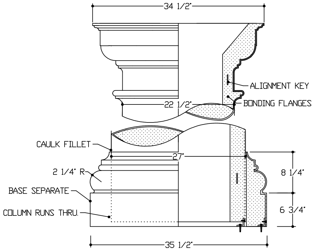
BASE ATTACHMENT DETAILS
