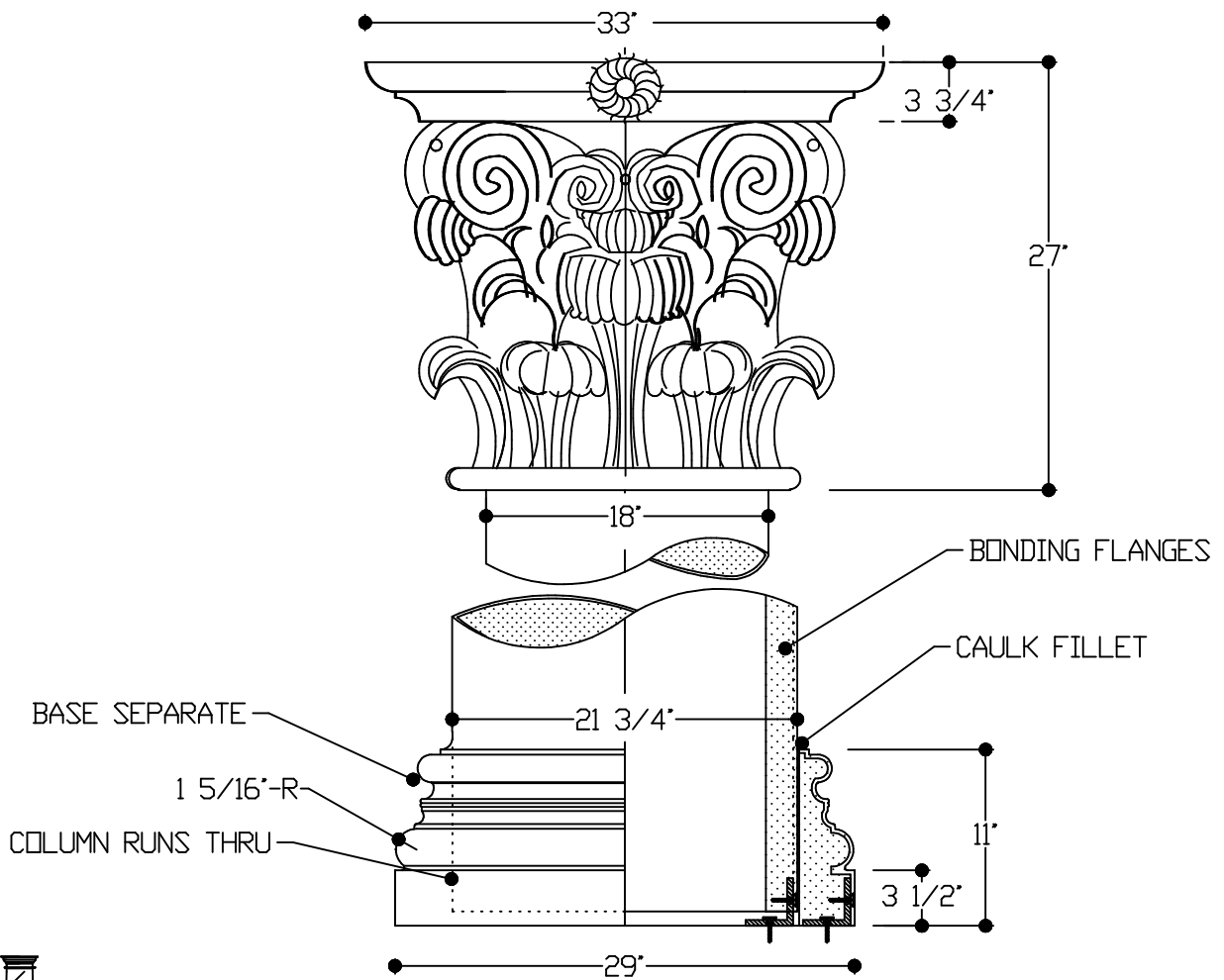
BASE ATTACHMENT DETAILS
