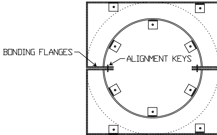
BASE ATTACHMENT DETAILS
