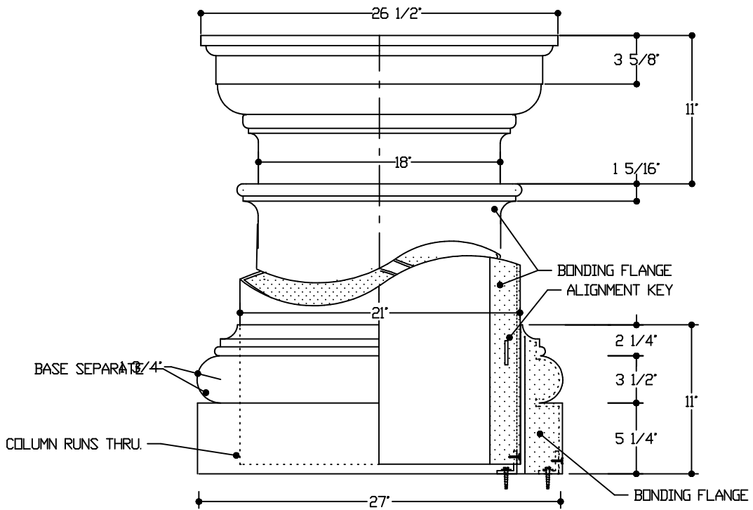
BASE ATTACHMENT DETAILS
