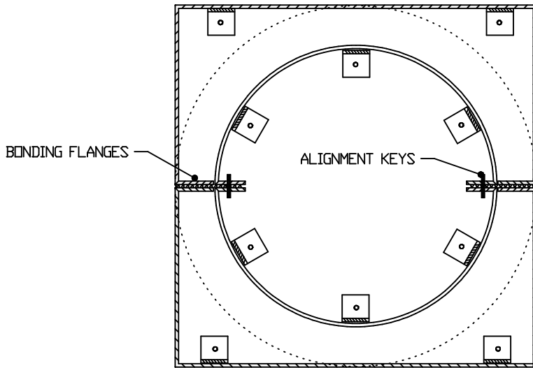
BASE ATTACHMENT DETAILS
