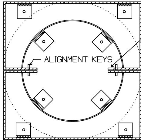
BASE ATTACHMENT DETAILS
