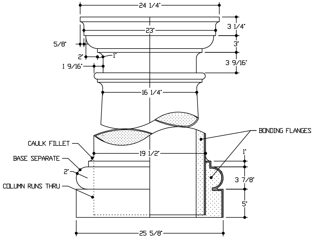
BASE ATTACHMENT DETAILS
