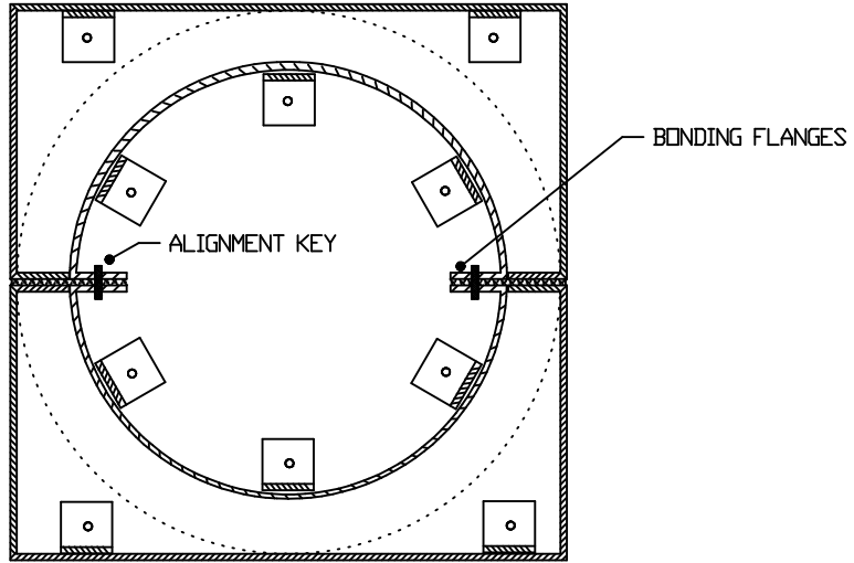
BASE ATTACHMENT DETAILS
