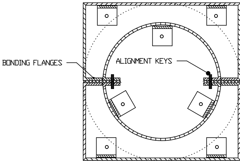
BASE ATTACHMENT DETAIL
