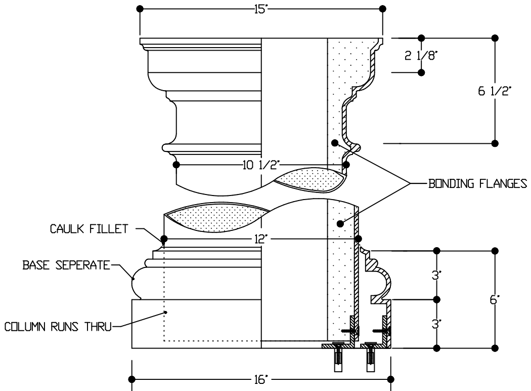
BASE ATTACHMENT DETAIL
